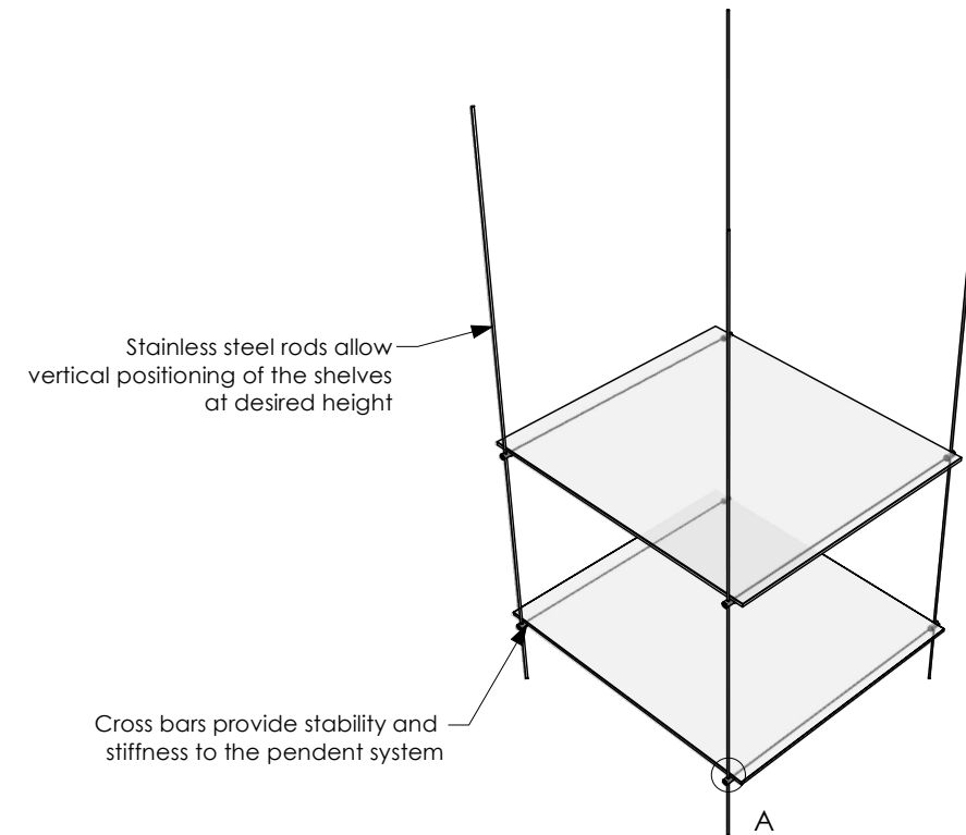
HANGING ROD SHELving
