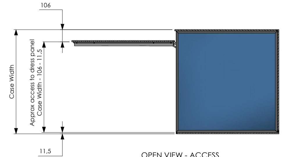
OPEN VIEW - ACCESS
