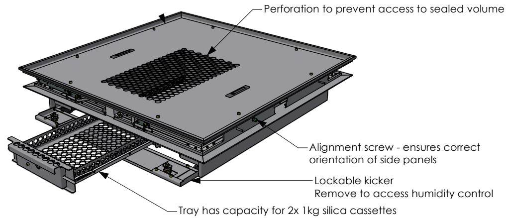
BOTTOM STRUCTURE (EXTERNALLY ACCESSED HUMIDITY CONTROL FACILITY)
